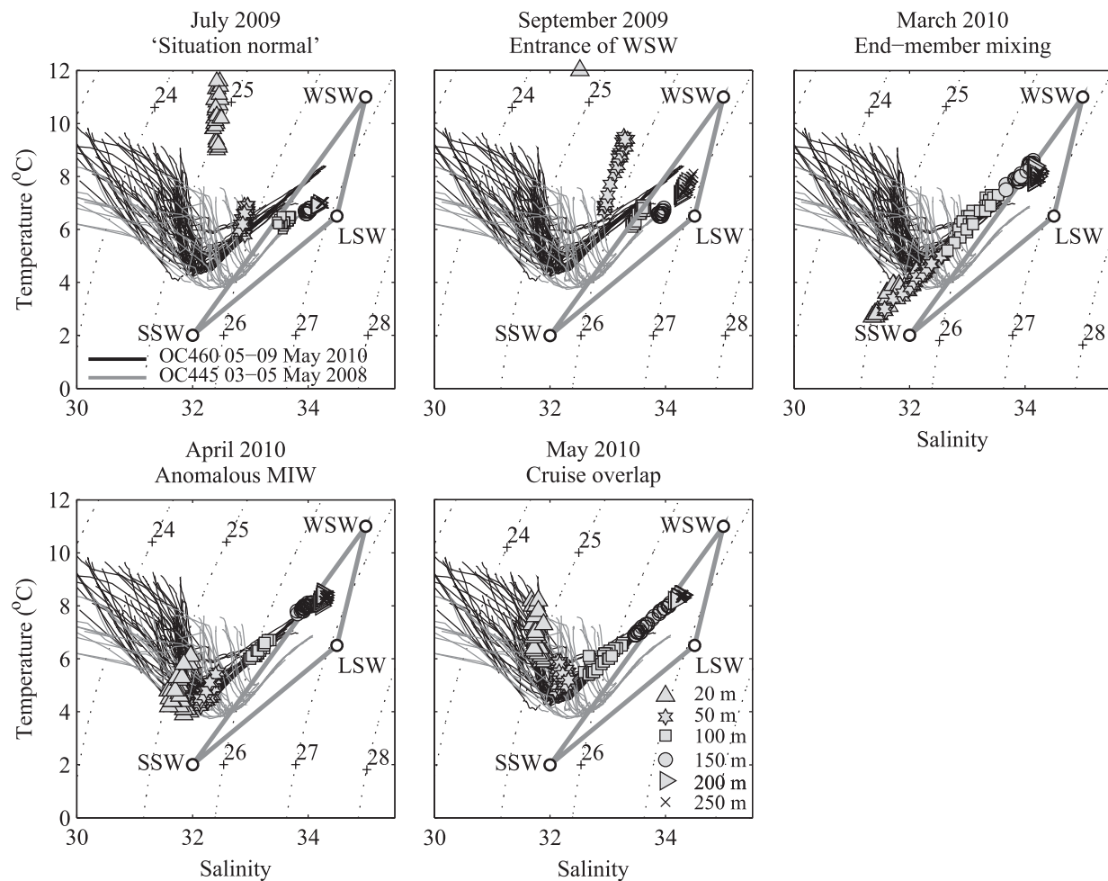
Fig. 14. Time-series of temperature–salinity diagrams from NERACOOS mooring M in Jordan Basin. Daily values are plotted in each month. Dotted lines are contours of \sigma -T density anomaly. Vertices of the mixing triangle consist of the canonical water-mass characteristics for Warm Slope Water (WSW), Labrador Slope Water (LSW), and Scotian Shelf Water (SSW) described in Smith et al. (2001).
