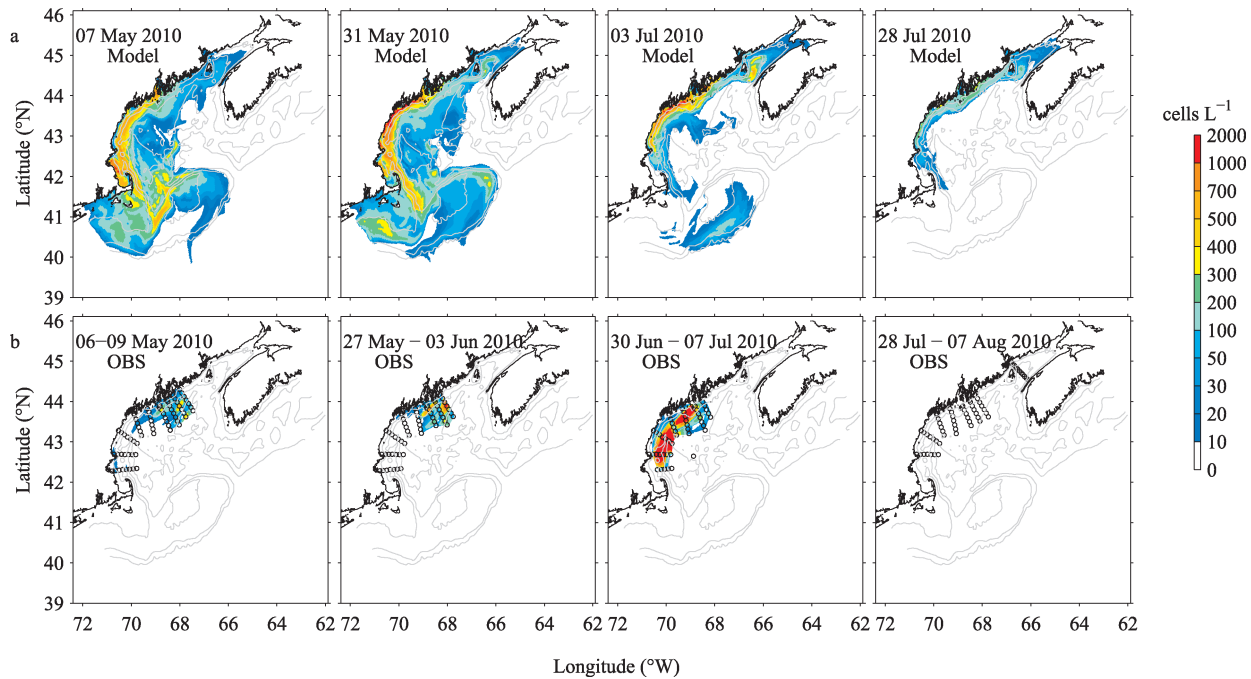
Fig. 5. (a) A. fundyense model predictions for 2010. For a complete description of the forecast system and 2010 results, see http://omglnx3.meas.ncsu.edu/GOMTOX/2010forecast/ . (b) Observations for early May, late May–early June, late June–early July, and late July–early August. Note that the cell-count maps include all available stations (open circles), whereas the hydrographic comparisons in Figs. 6–10 only include those stations in common with all (transects T1–T5 in Fig. 1).
