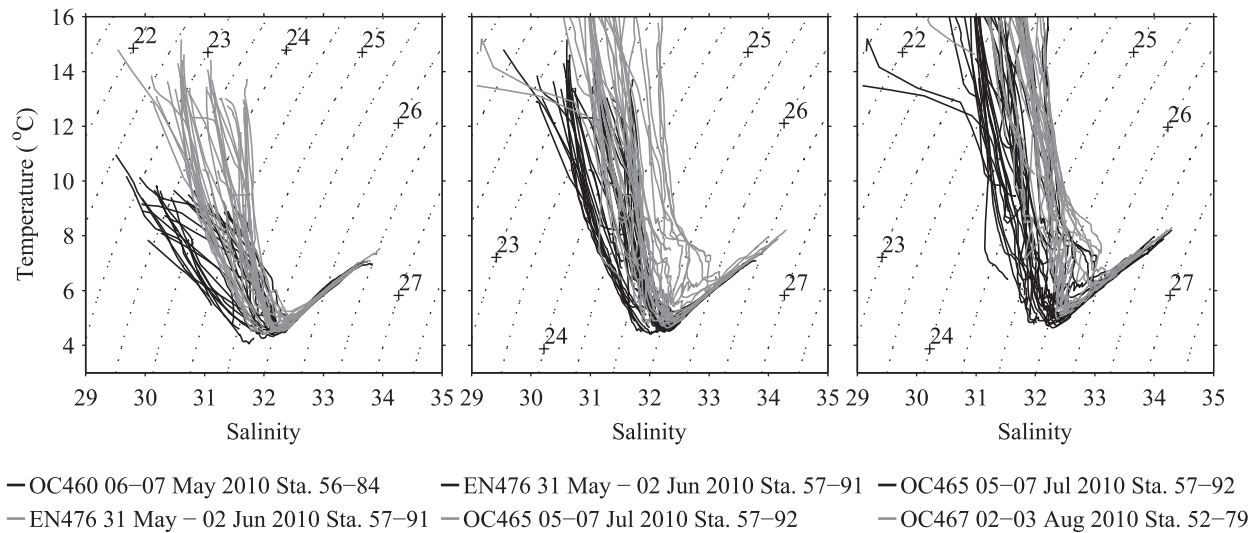
Fig. 8. Seasonal variability in water mass characteristics in the western Gulf of Maine during spring-summer 2010. Four time intervals are documented: 06-07 May, 31 May-02 June, 05-07 July, and 02-03 August. In each panel, the earlier cruise is shown in black and the later cruise in grey. Dotted lines are contours of sigma-T density anomaly.
